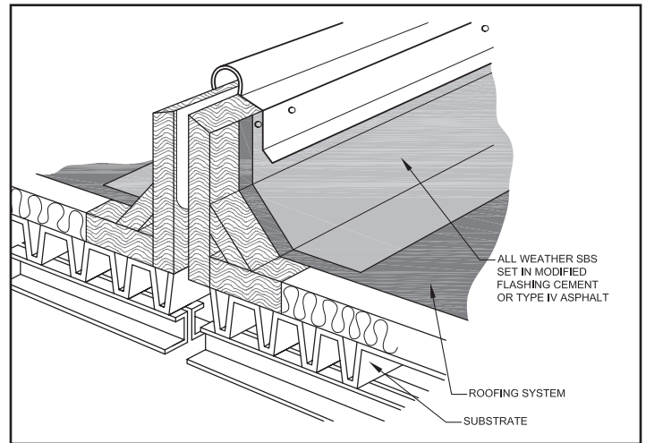
All Weather SBS Detail 10 Roof Projection
