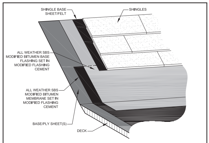
All Weather SBS Detail 12 Flat Roof/Shingle Tie-in
