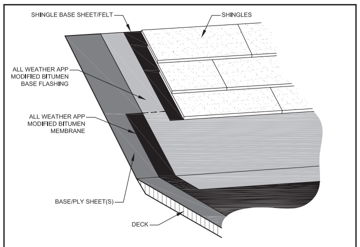
All Weather APP Detail 12 Flat Roof/Shingle Tie-in
