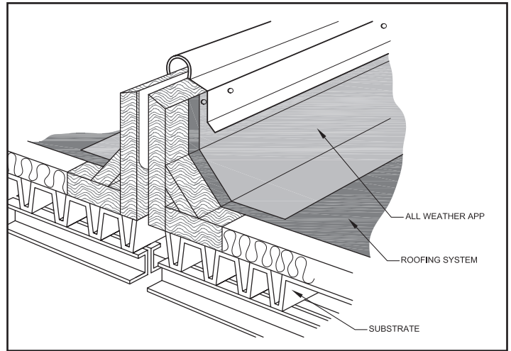
All Weather APP Detail 10 Roof Projection
